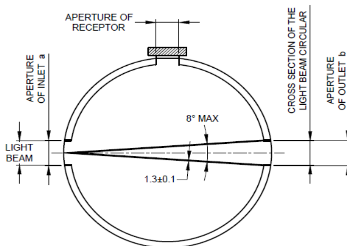
FIG. 2 CONDITIONS OF THE INTEGRATION BALL
